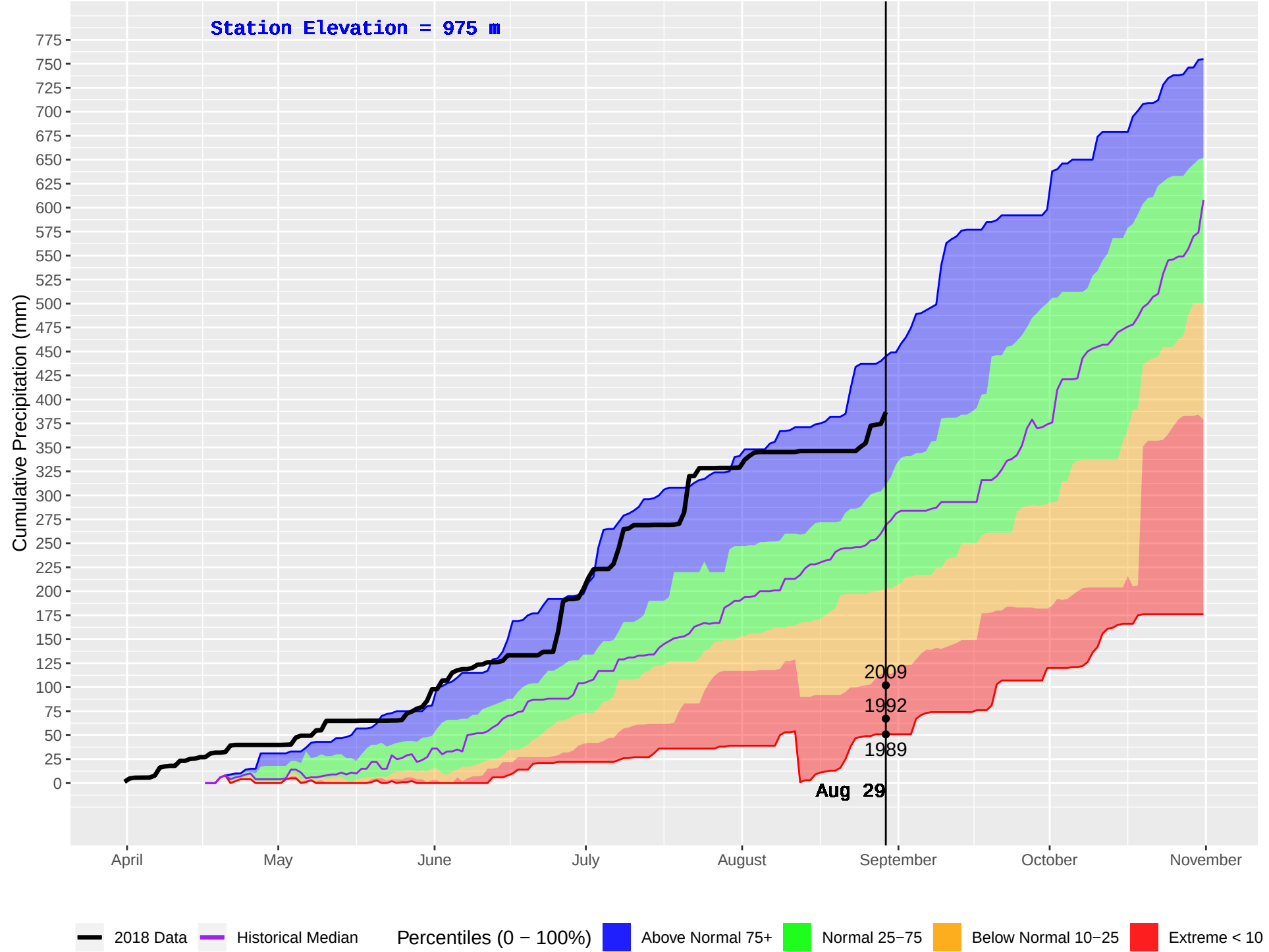
MCGREGOR 2 (192) : Historical (1986–2016) and Current (2018) Daily Cumulative Precipitation
