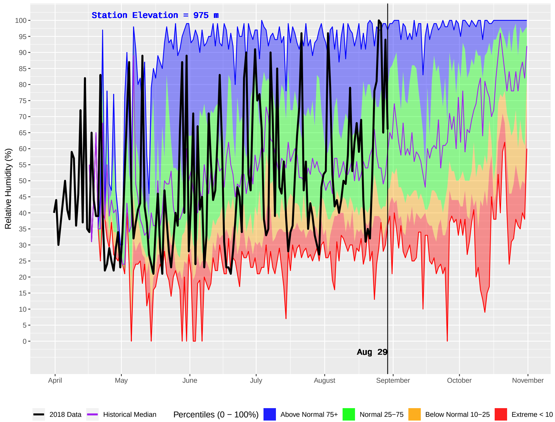
MCGREGOR 2 (192) : Historical (1986–2016) and Current (2018) Daily Relative Humidity
