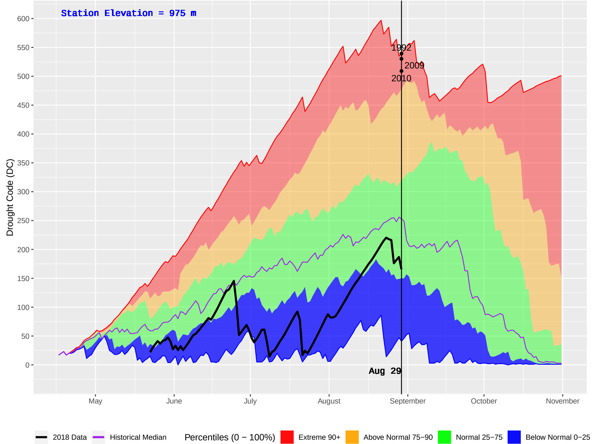
MCGREGOR 2 (192) : Historical (1986–2016) and Current (2018) Daily Drought Code (DC)
