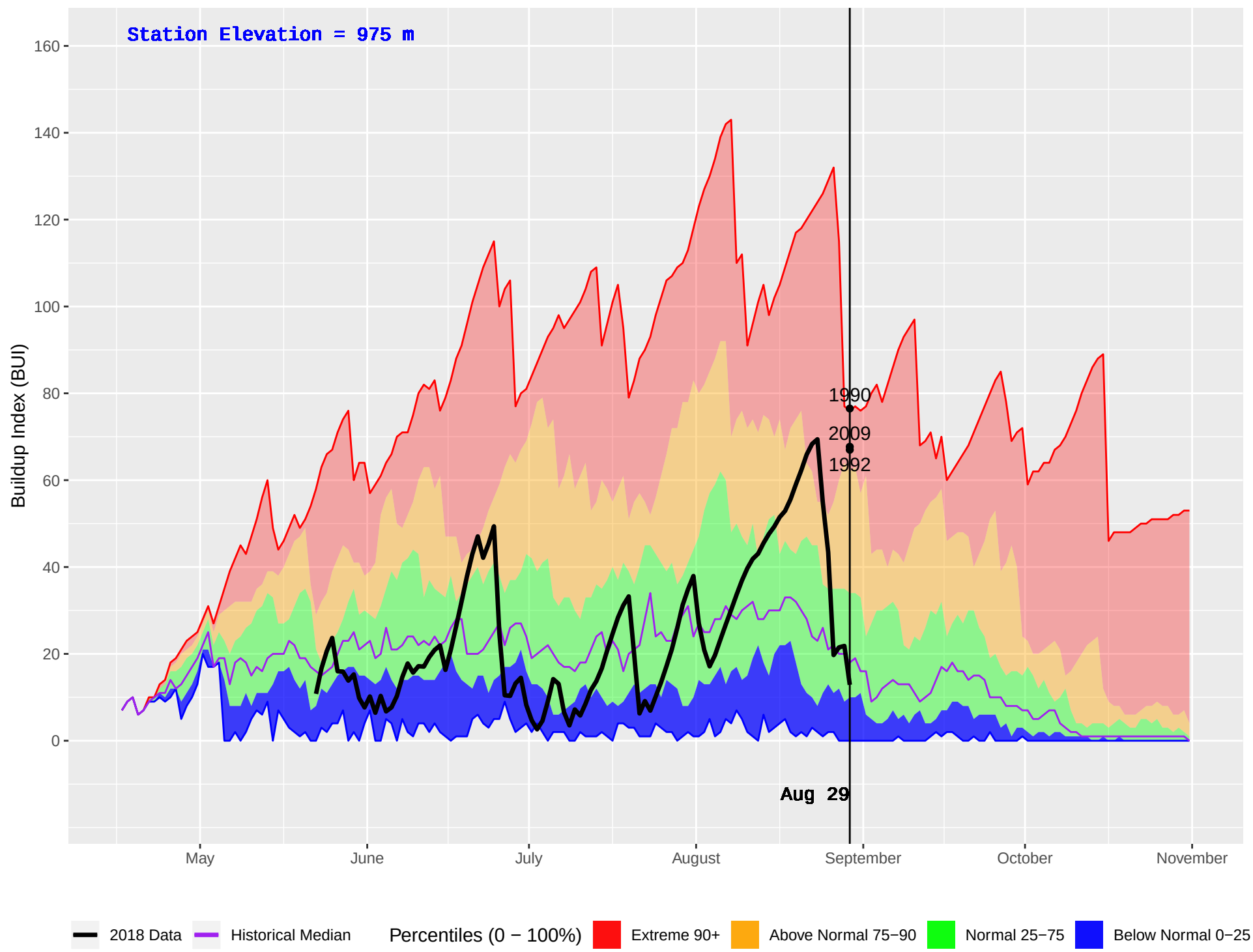
MCGREGOR 2 (192) : Historical (1986–2016) and Current (2018) Daily Buildup Index (BUI)
