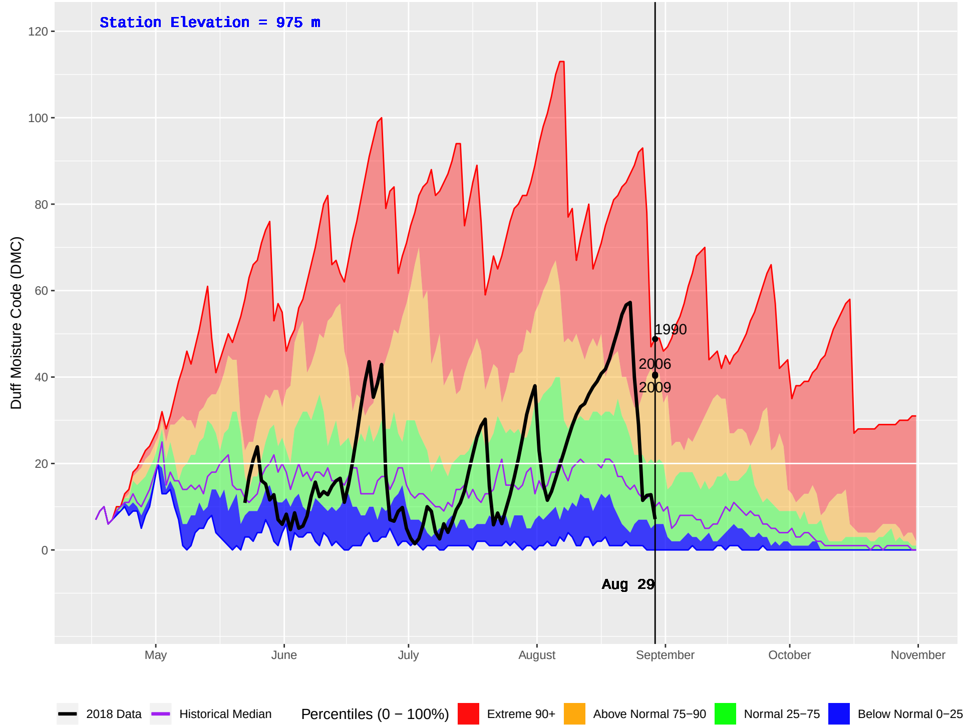
MCGREGOR 2 (192) : Historical (1986–2016) and Current (2018) Daily Duff Moisture Code (DMC)
