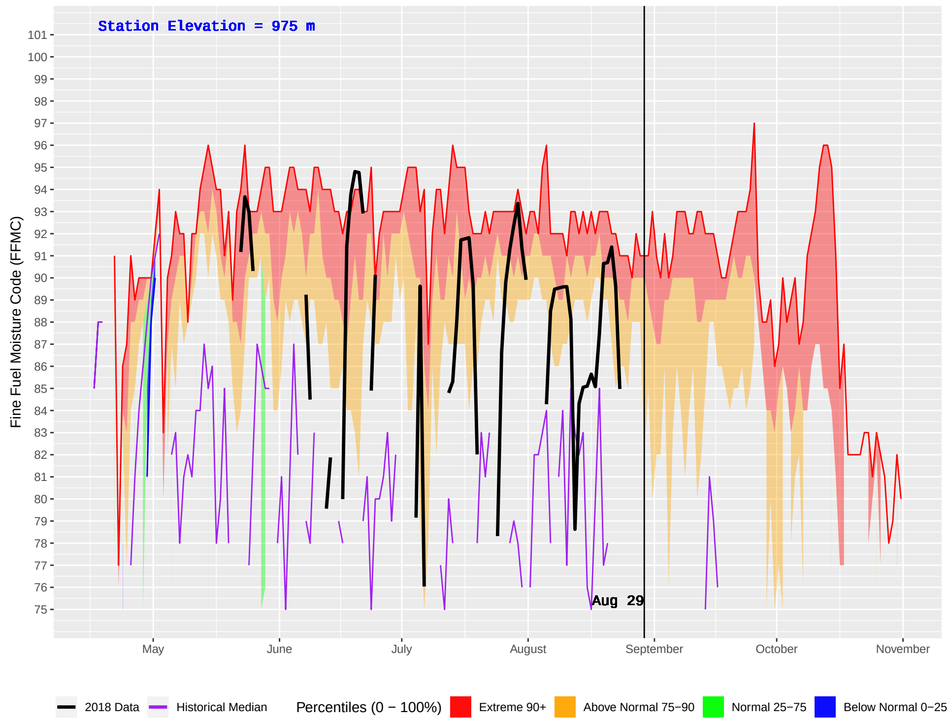
MCGREGOR 2 (192) : Historical (1986–2016) and Current (2018) Daily Fine Fuel Moisture Code (FFMC)
